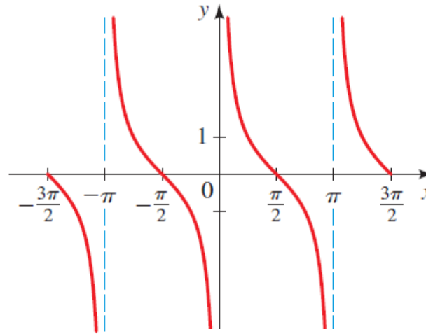
y = \cot x
