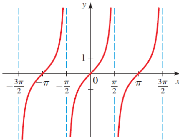
y = \tan x
